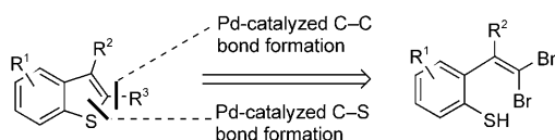
Scheme 1. Retrosynthetic strategy.
